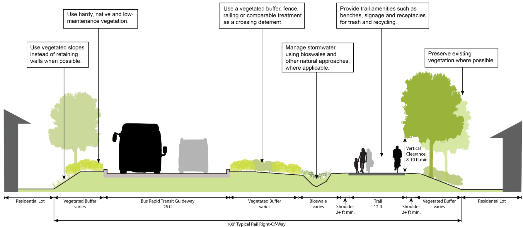
Figure 5: Proposed Dedicated Guideway and Bruce Vento Trail in the Ramsey County Rail Right-of-Way at the Typical 100-Foot Right-of-Way Segment
