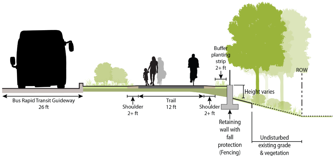
Figure 61: Retaining Wall Strategy
