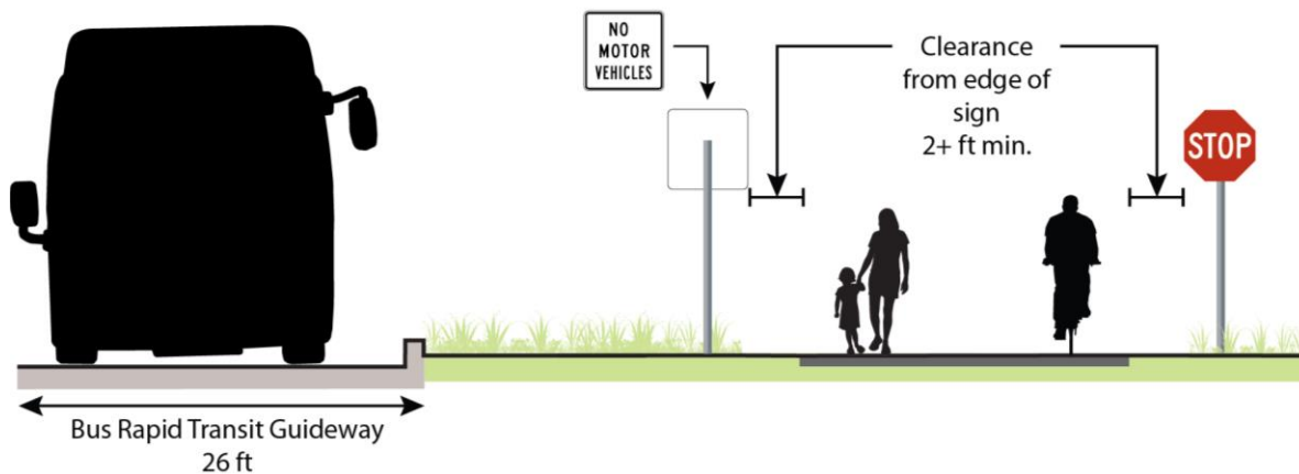
Figure 50: Typical Signage at Roadway Crossings
