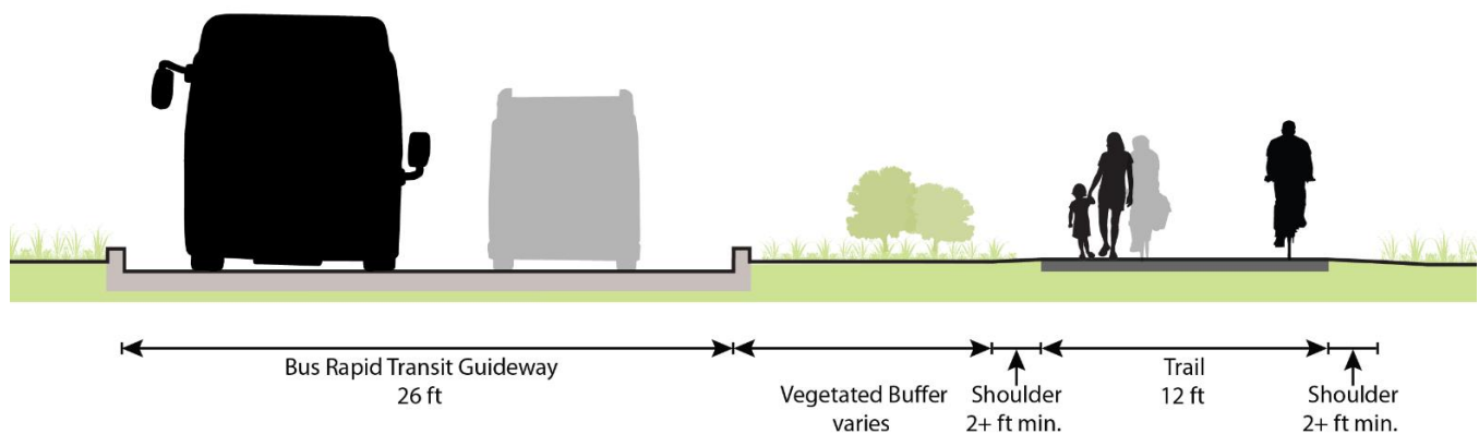
Figure 39: Typical BRT and Trail Section
