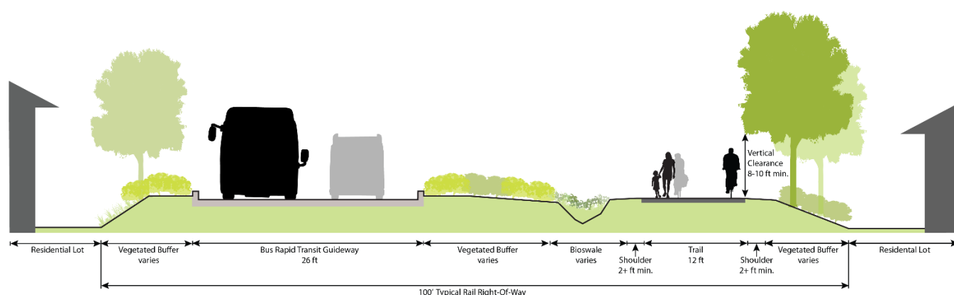
Figure 42: Typical Buffer and Screening Treatment
