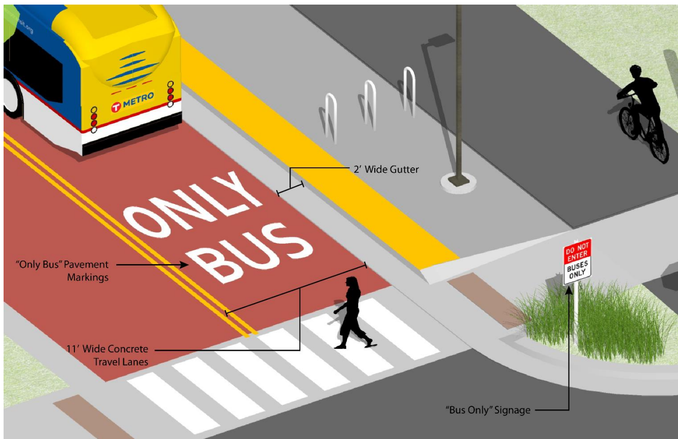
Figure 38: Typical Dedicated Guideway Dimensions
