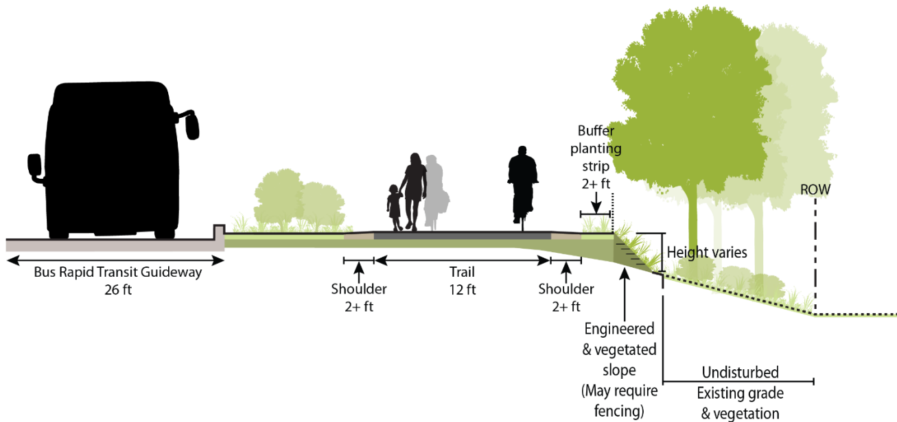
Figure 60: Engineering and Vegetative Slope Strategy
