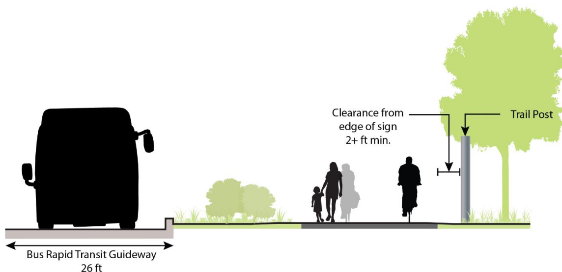
Figure 58: Typical Trail Post
