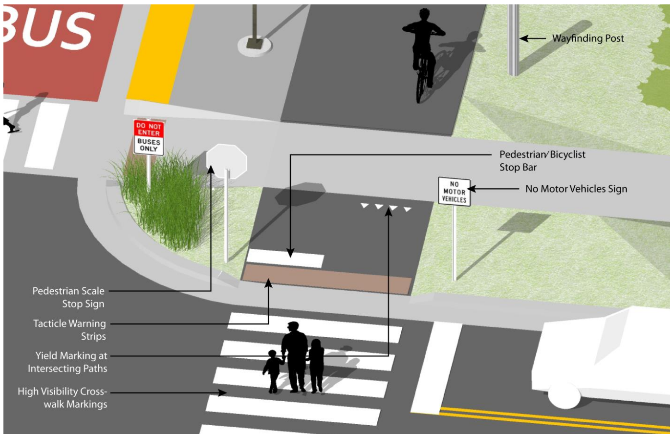
Figure 51: Typical Signage and Markings at Roadway Crossings
