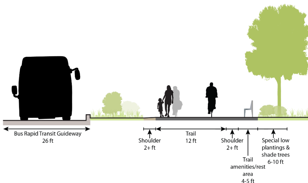
Figure 56: Trail Amenity/Rest Area
