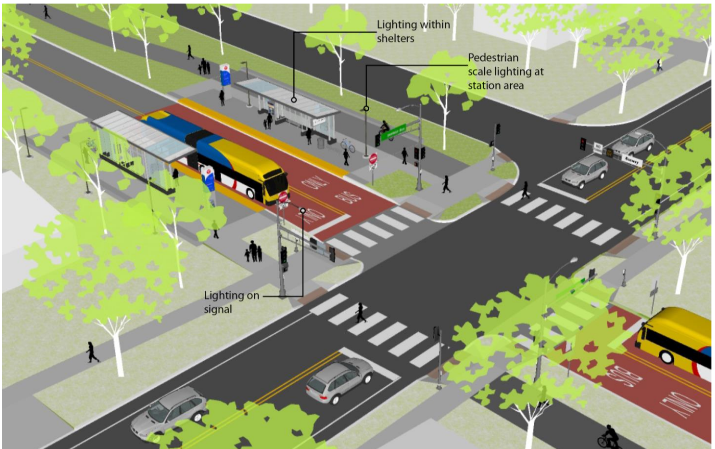
Figure 48: Potential Intersection Lighting Strategy
