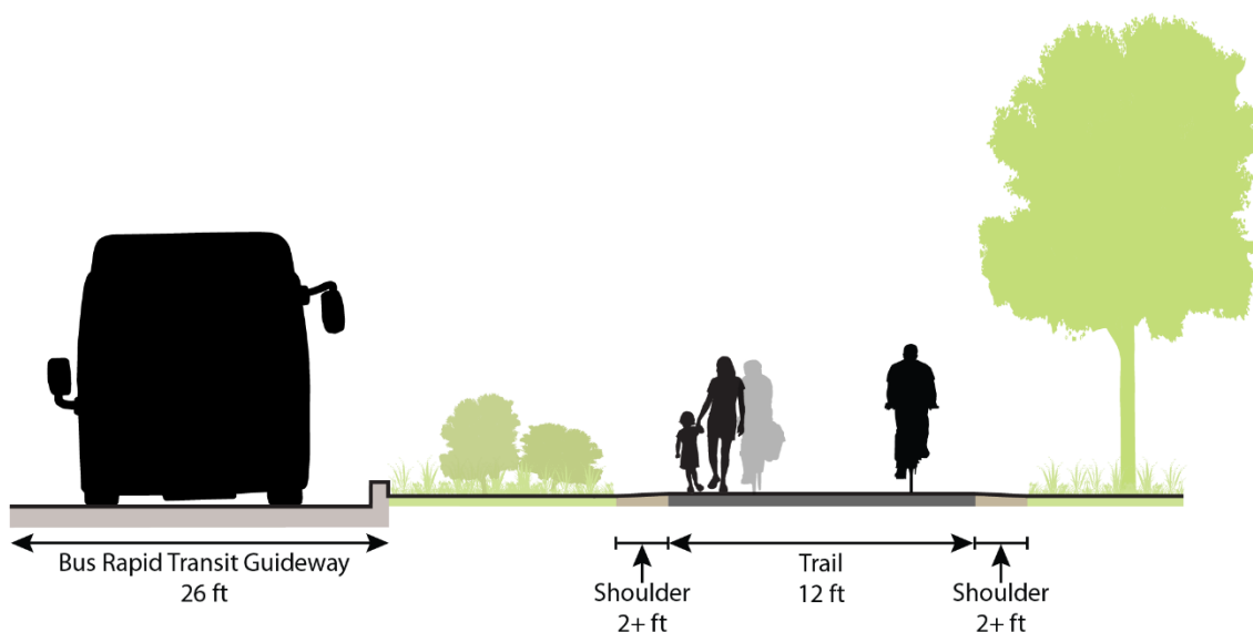
Figure 37: Typical Trail Section
