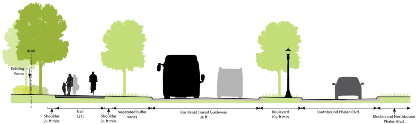
Figure 36: Typical BRT and Trail Section Along Phalen Boulevard
